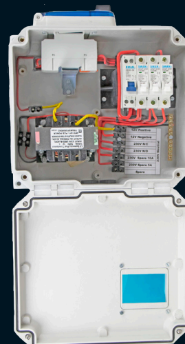
“Stand Up” Pool Box™ with transformer
